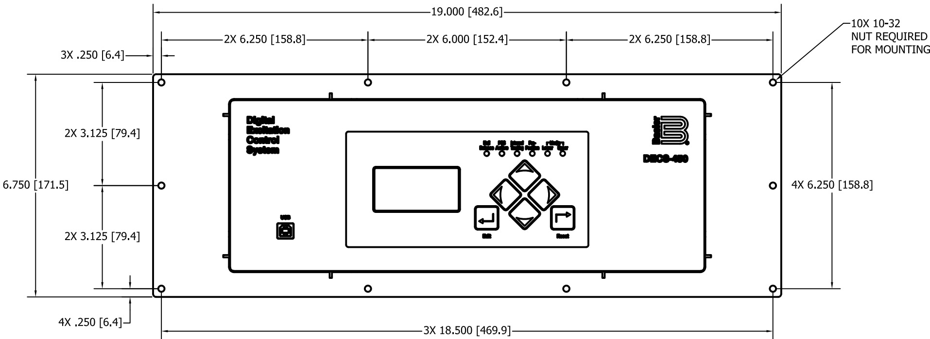
DECS-300 CONVERSION
