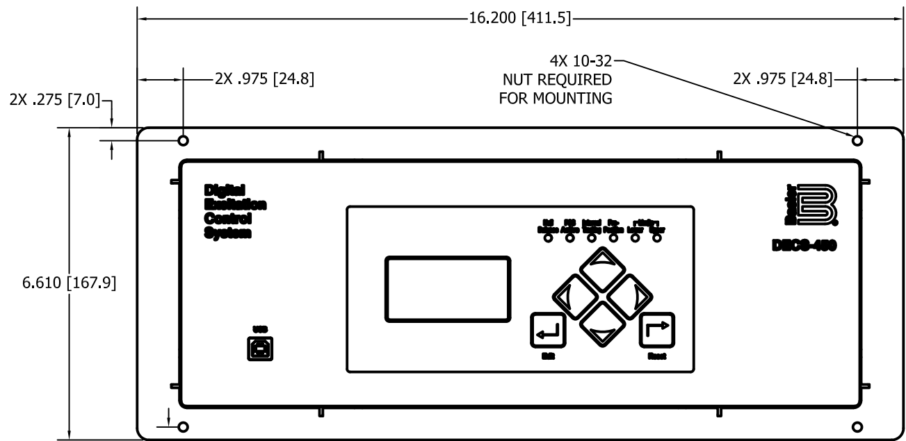
ESCUTCHEON PLATE
